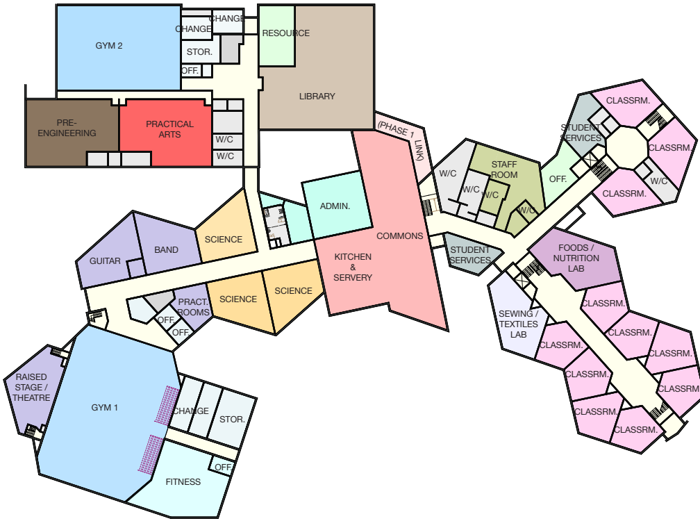
CONCEPT A - MAIN LEVEL
