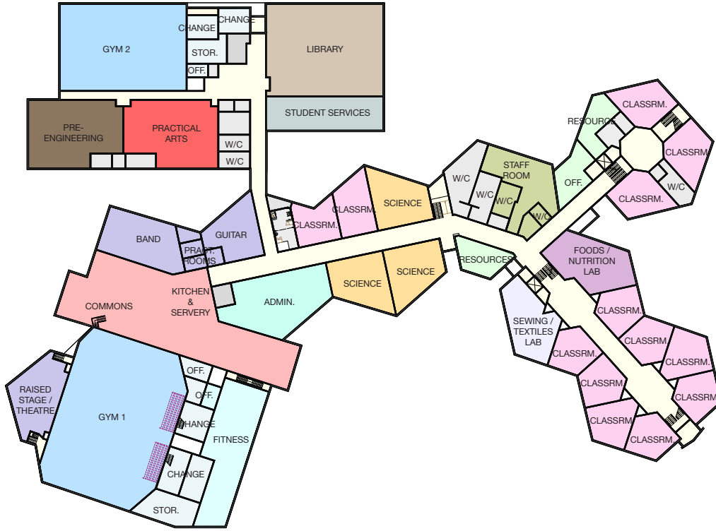
CONCEPT B - MAIN LEVEL
