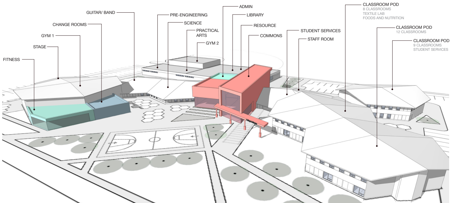
CONCEPT A - 3D MASSING
